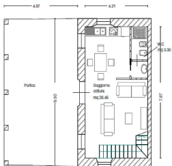
Piano Seminterrato
