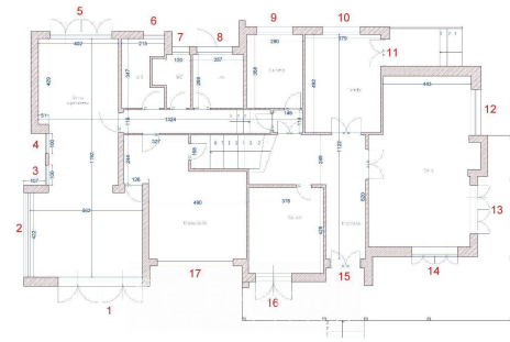
Piano Terra
